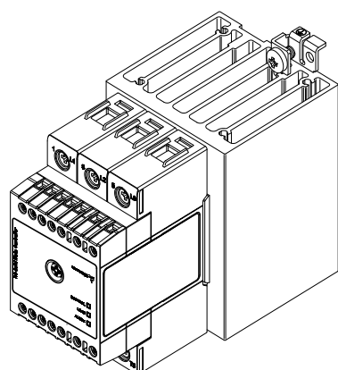
RGC2..I40, RGC2..V40 RGC3..I30, RGC3..V30
